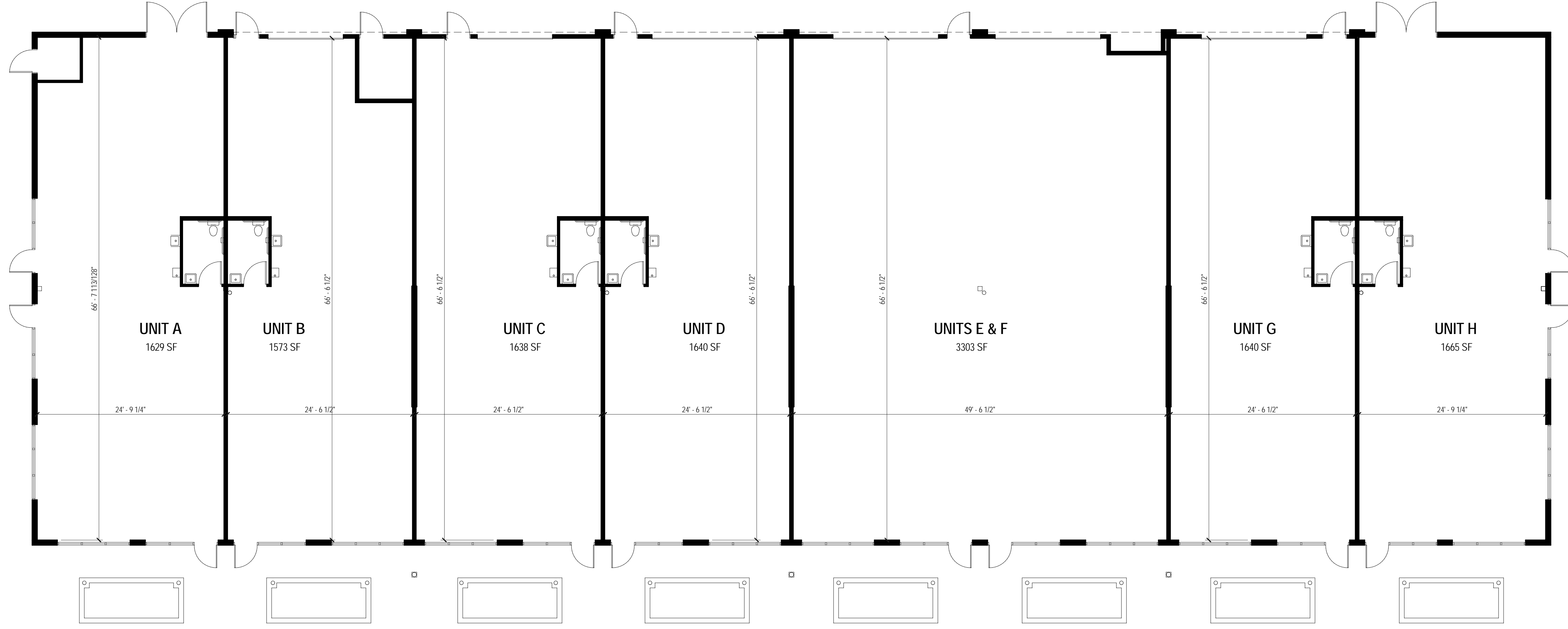
1 BUILDING 6410 1/8" = 1'-0"
